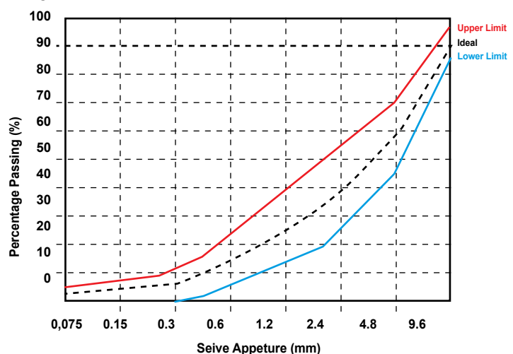
Chart 8-4: Grading limits envelope
