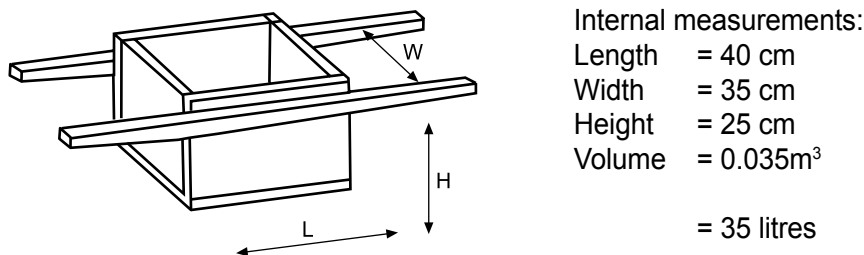
Figure 7-1: Concrete gauge box
