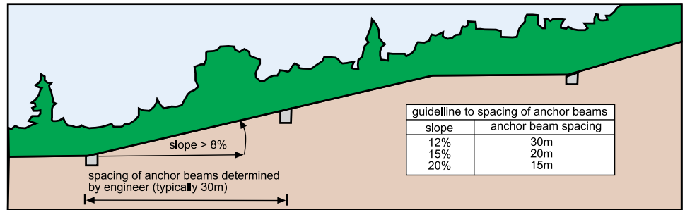
Figure 8-17: Spacing of anchor beams
