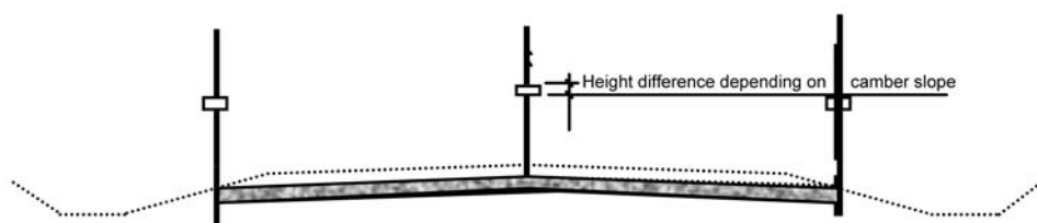
Figure 5-3: Paved road camber formation
