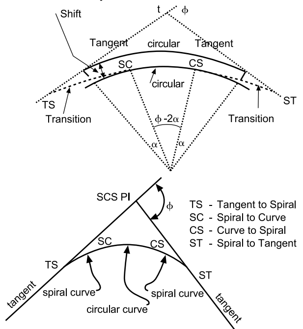
Figure 3-35: Transition curve
