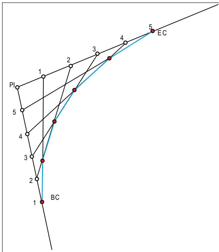
Figure 3-24: The string line method
