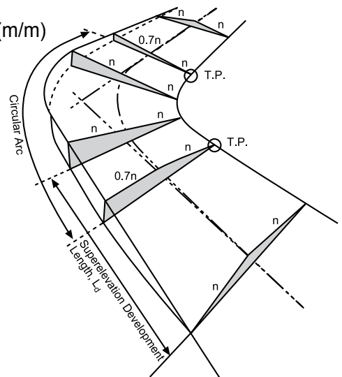
Figure 3-34: Development of superelevation on curves curve
