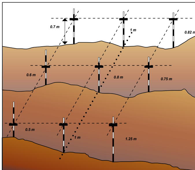
Figure 3-7: Transferring heights
