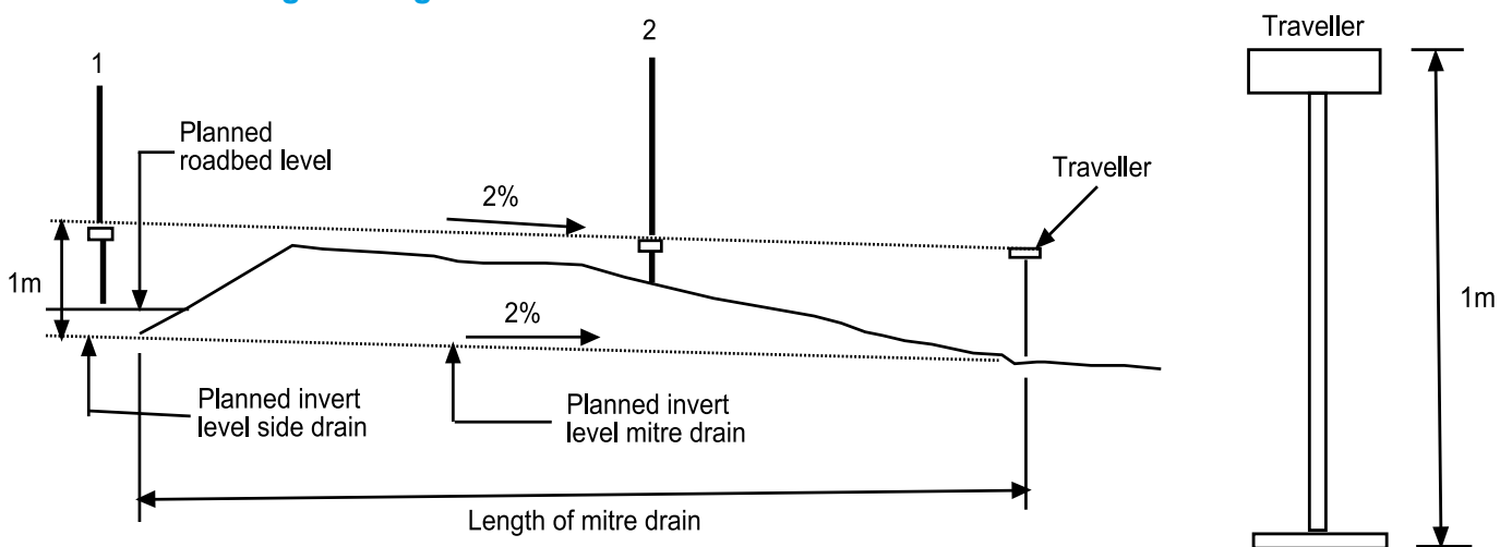
Figure 6-3: Checking the length of a mitre drain
