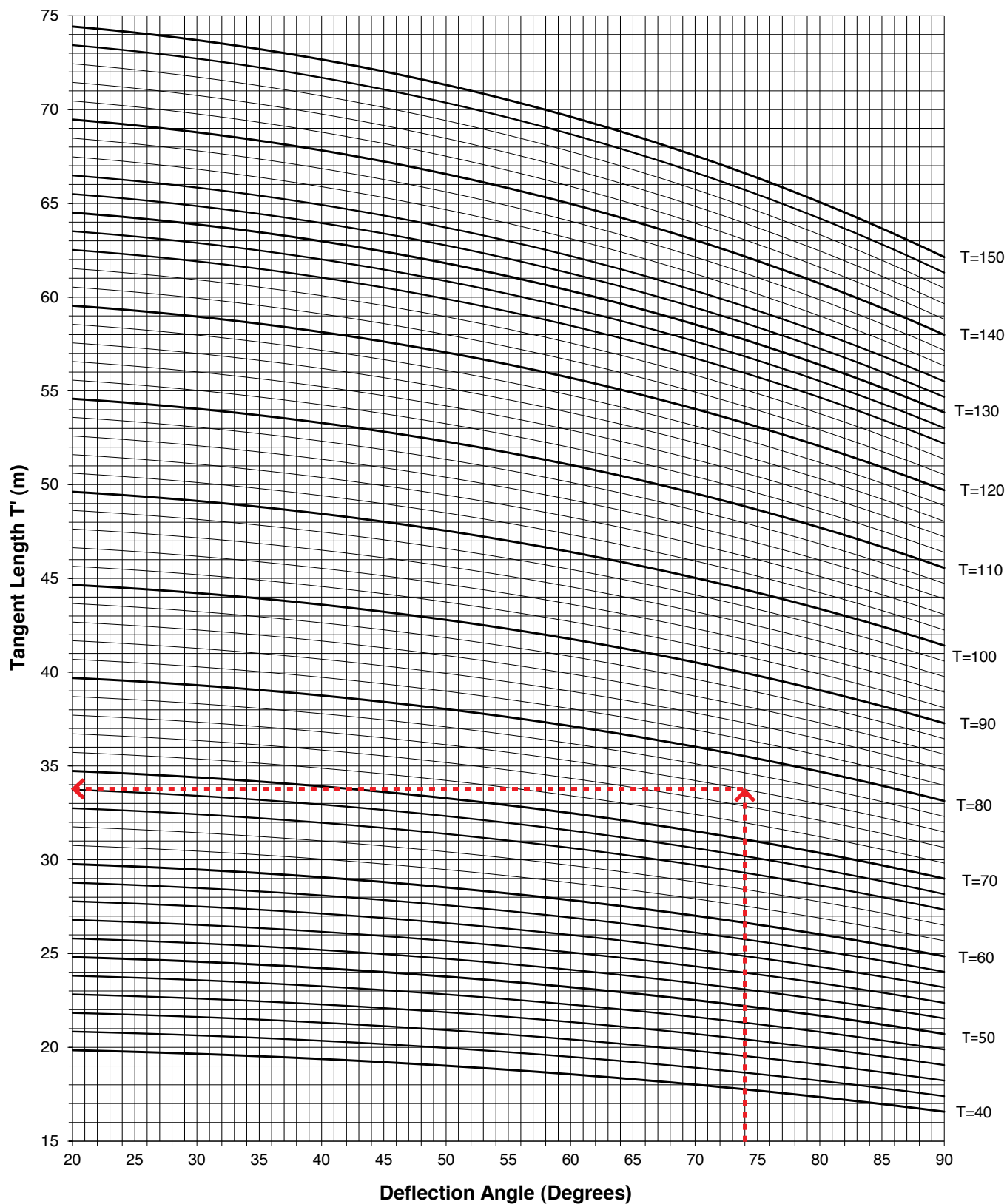
Tangent Length T' as a function of Deflection Angle and Curve Radius
