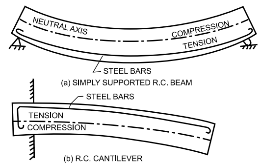
Figure 7-3: Reinforced concrete beams in tension and compression
