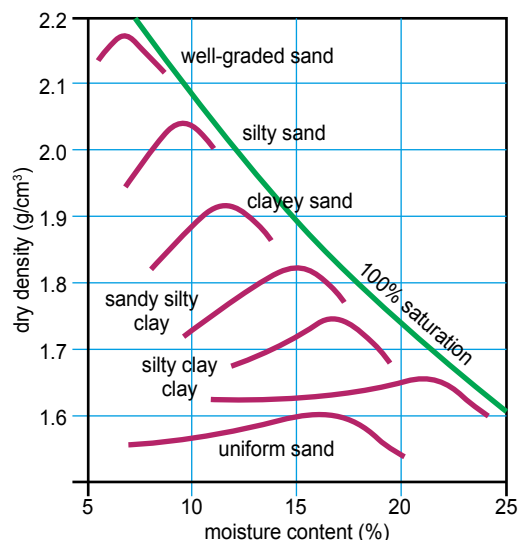
Chart 5-3: Moisture content – dry density
