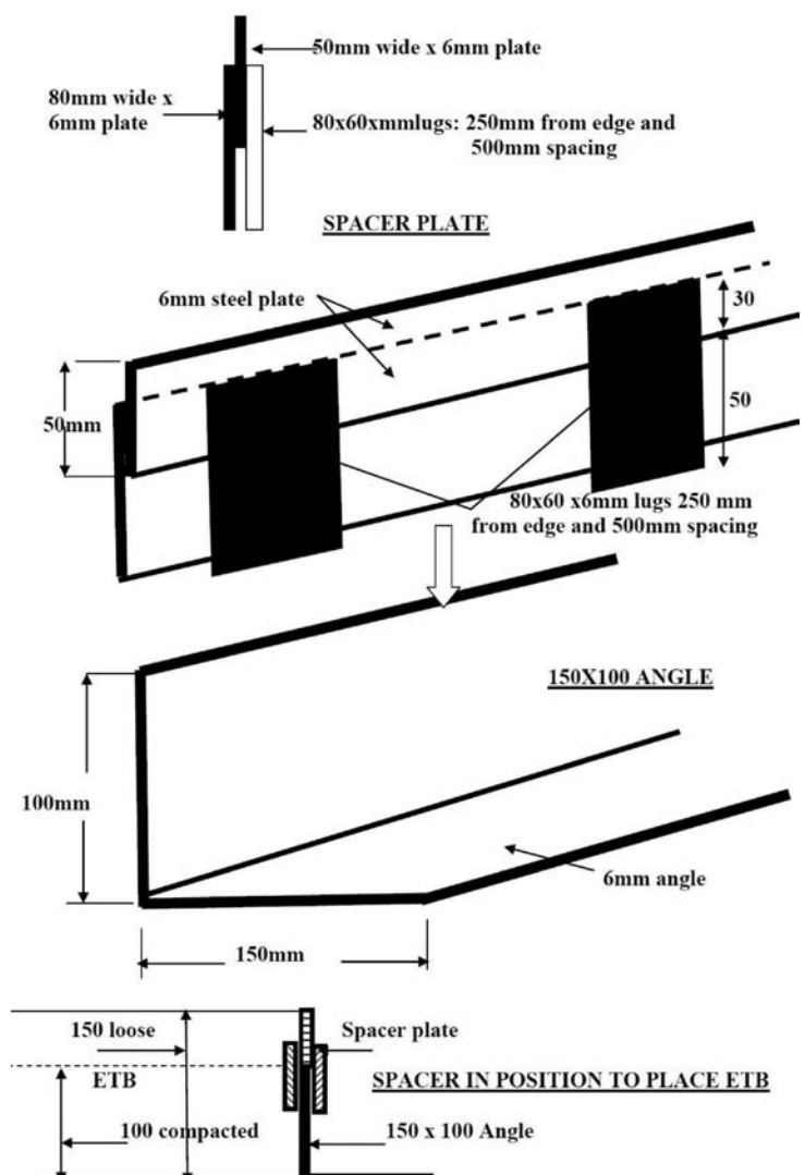
Figure 5-9: Shutter arrangement for ETB
