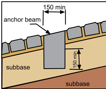
Figure 8-16: Typical section through anchor beam showing dimensions
