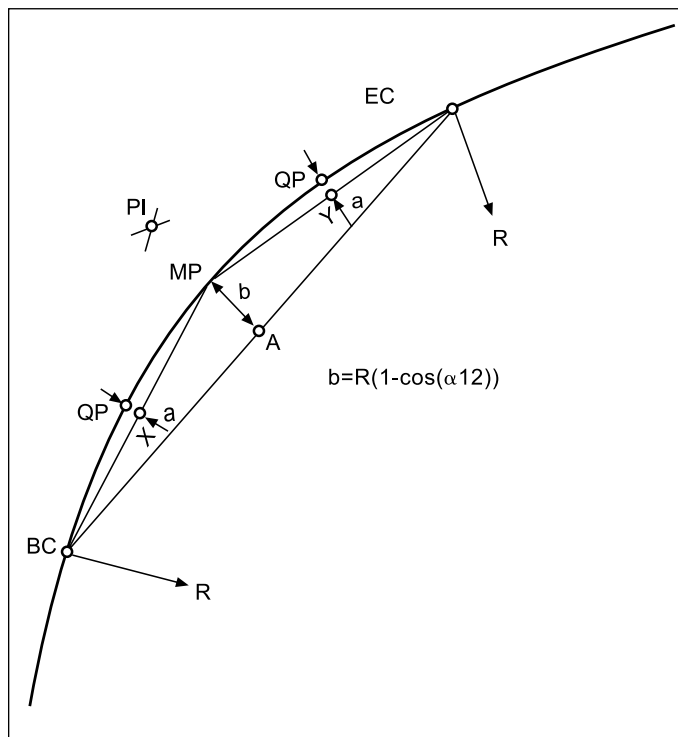
Figure 3-21: Setting out using the quarter method
