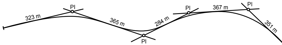
Figure 3-14: Horizontal curves connecting straight centrelines
