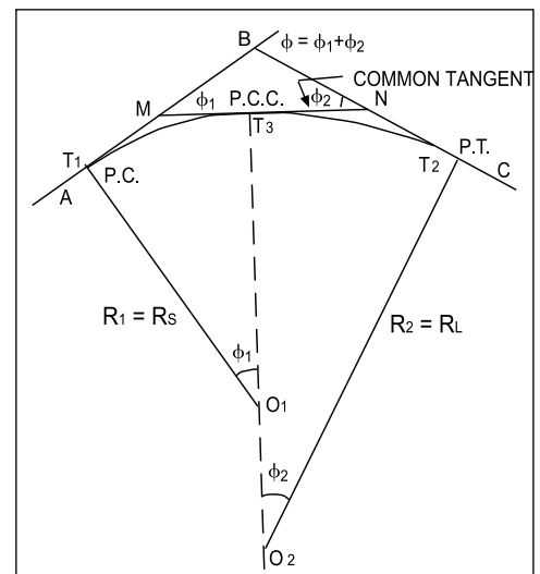
Figure 3-31: Compound curves
