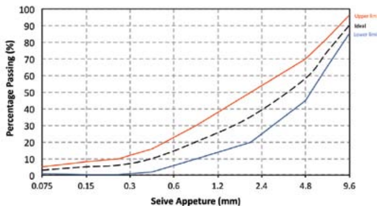
Chart 8-2: Grading limits envelope
