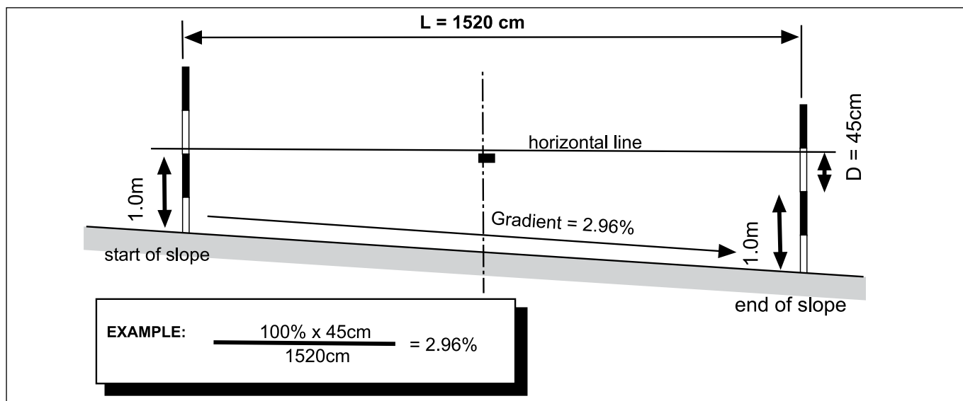
Figure 3-12: Confirming gradients
