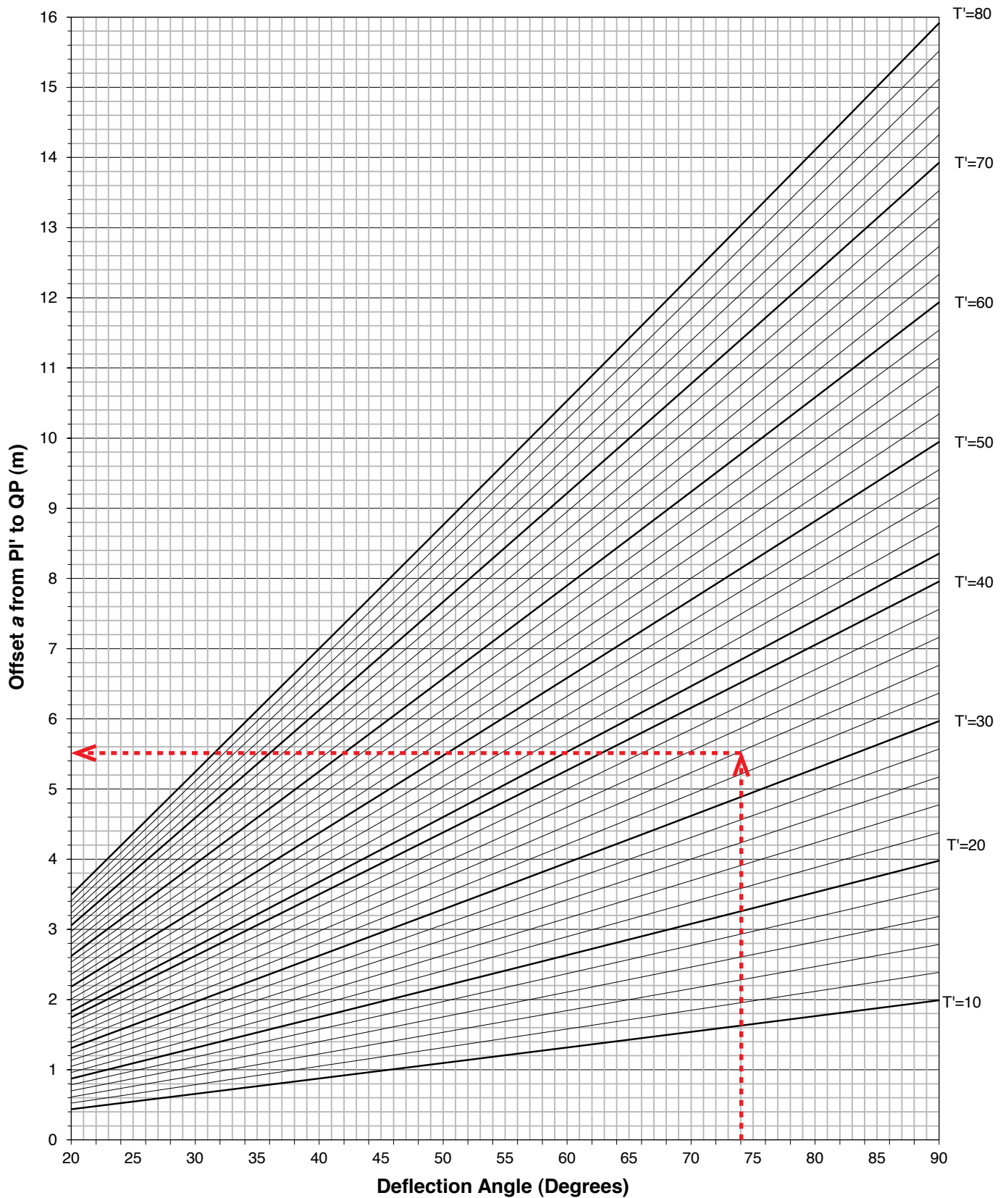
Offset a from PI' to QP as a function of tangent T'
