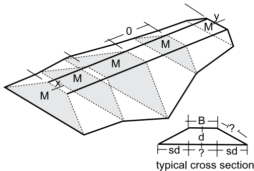
Figure 4-9: Prismoidal method
