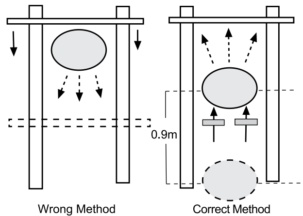
Figure 8-12: Spreading asphalt
