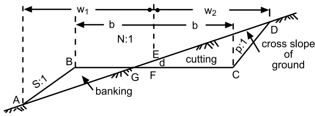
Figure 4-10: Cross-section in part-cut, part fill
