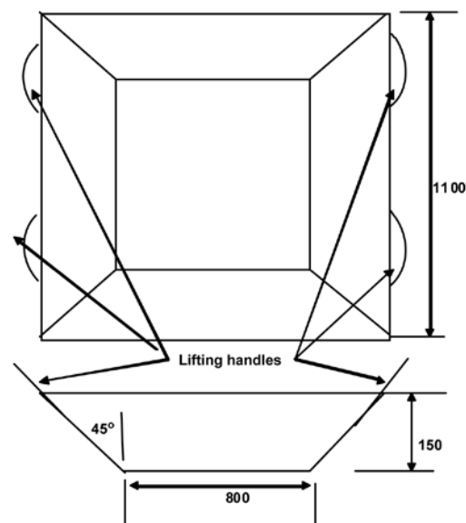
Figure 8-10: Drawing of steel tray
