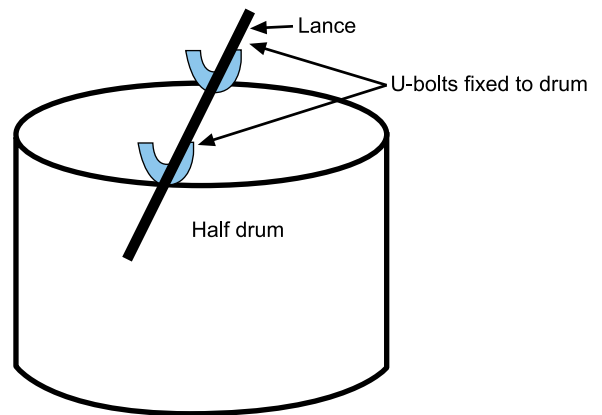
Figure 8-2: Rack for spray lance
