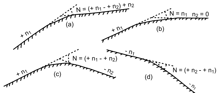
Figure 3-37: Crest curves
