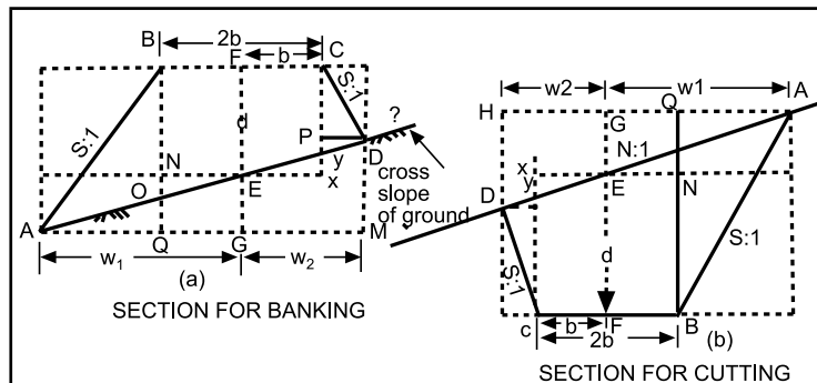
Figure 4-12: Full embankment or cut area
