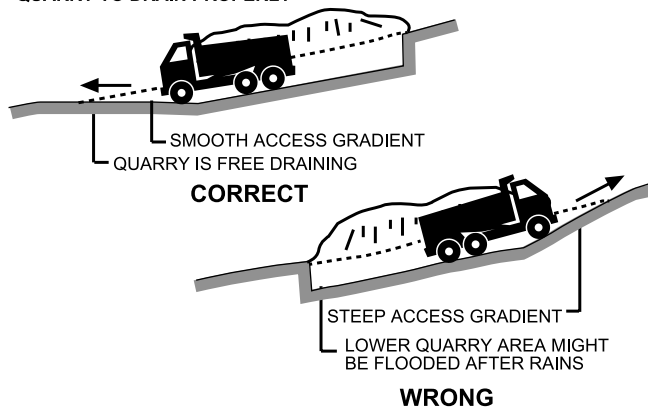
Figure 4-18: Quarry drainage
