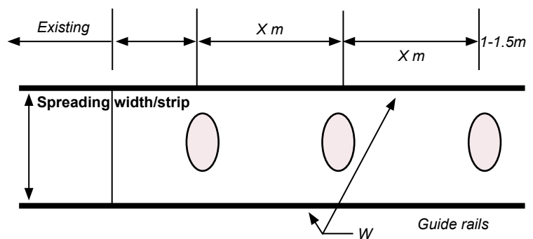
Figure 8-11: Spreading strip
