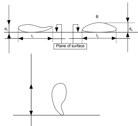
Figure A 7: Average Least Dimension of aggregate (ALD)
