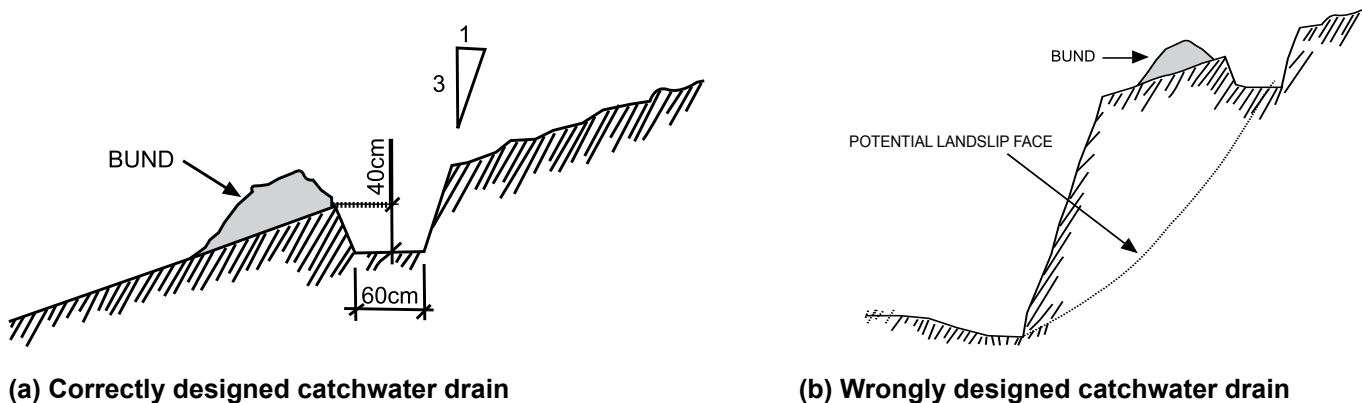
Figure 6-4: Catchwater Drain
