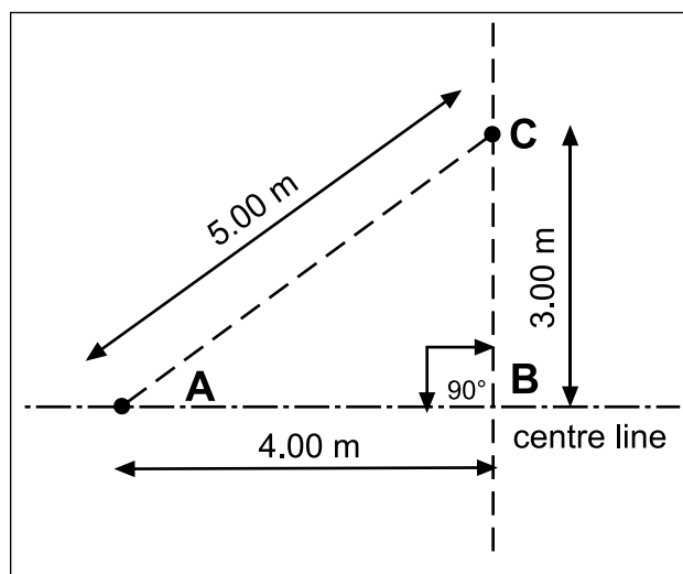
Figure 3-8: : Setting out of a 90° angle
