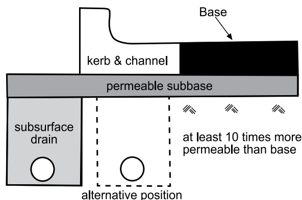
Figure 6-15: Cross-section of typical subsoil drains
