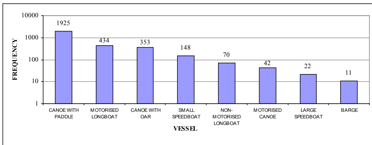
Graph 1: Vessel Frequency
