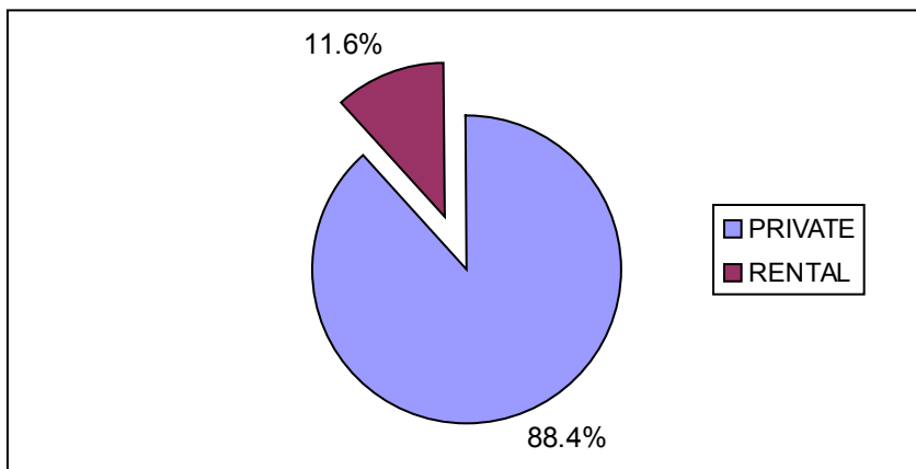
Graph 8: Vessel Ownership
