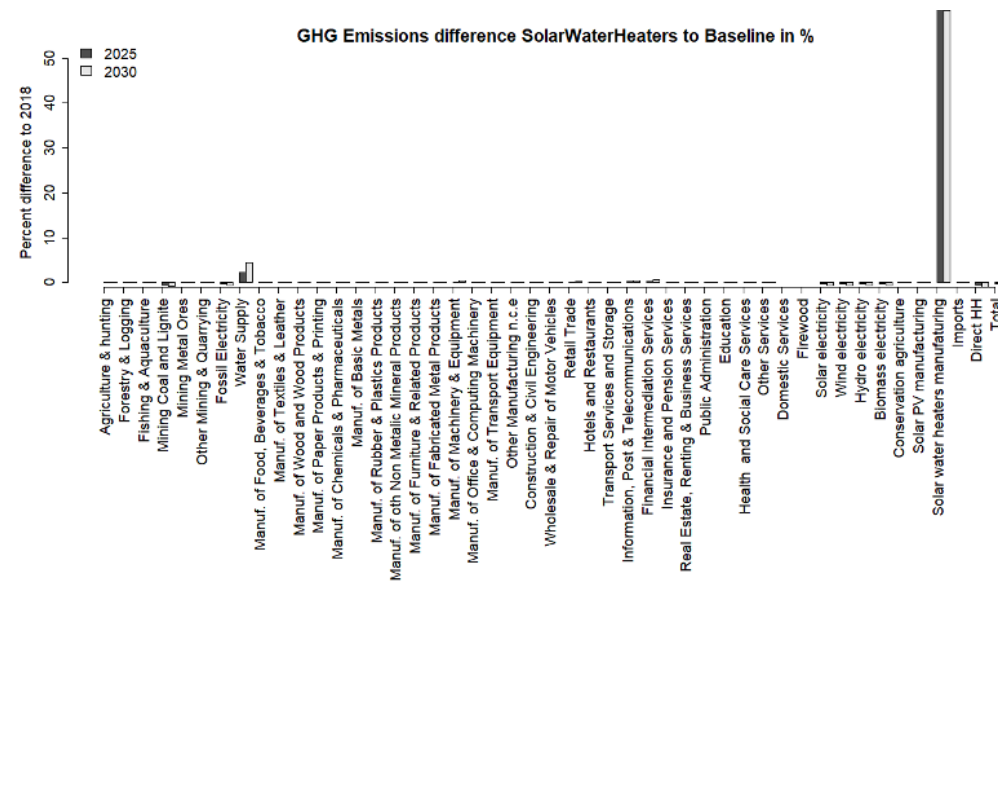
Figure 25: Solar water heater scenario compared to Baseline: GHG emissions by industry
