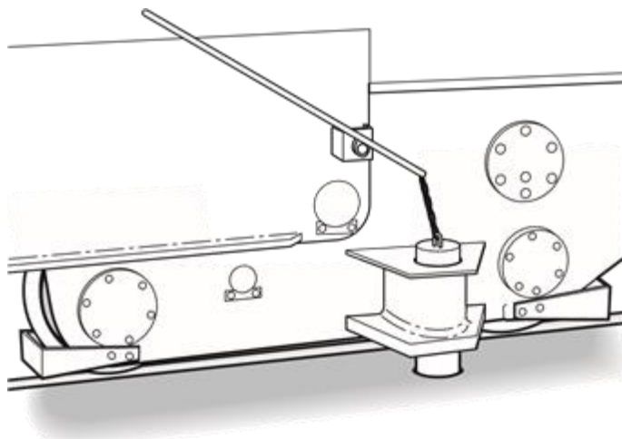
Figure 36. Storm pin on rail-mounted crane
