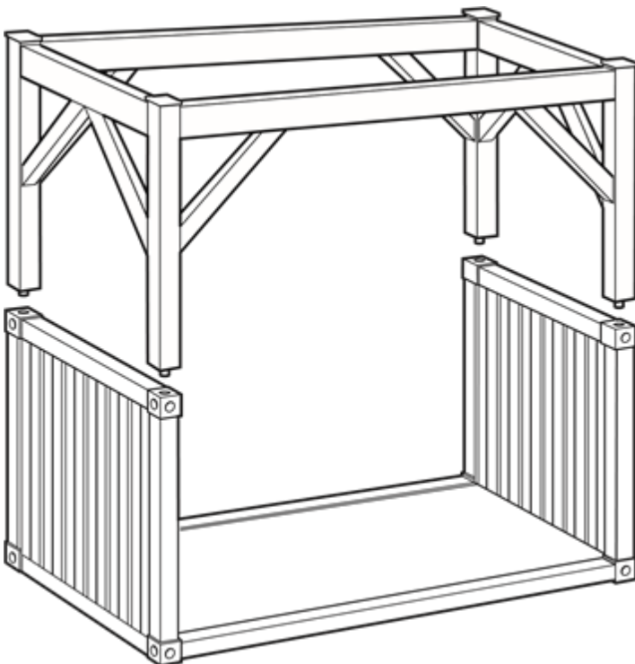
Figure 79. Over-height frame
