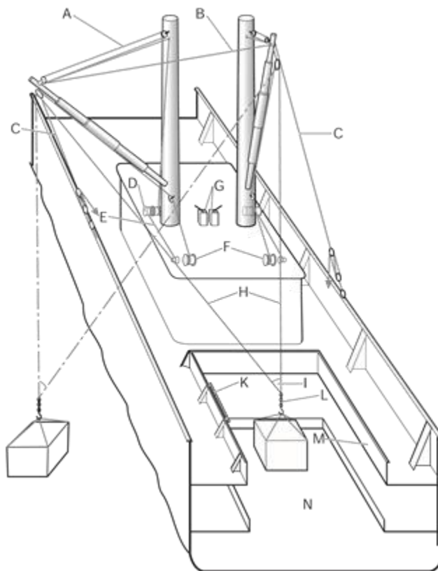
Figure 54. Derricks in union purchase rig
