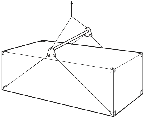
Figure 78. Bottom lifting of containers
