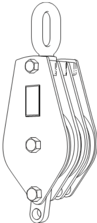
Figure 46. Three-sheave block with becket
