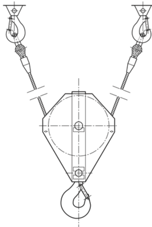
Figure 56. Equalizing pulley for two coupled cranes
