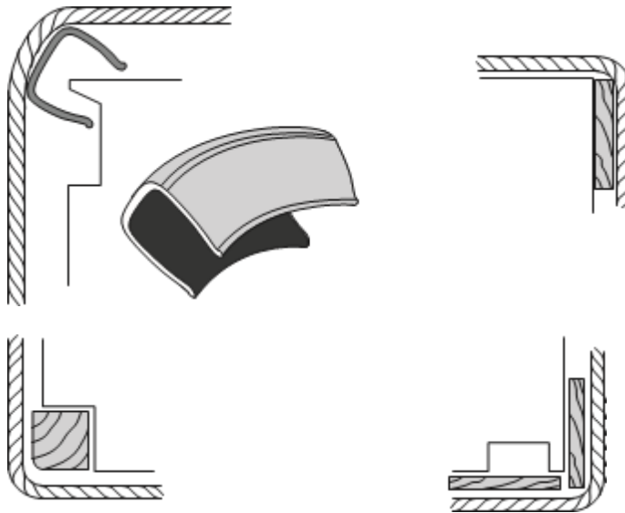
Figure 64. Methods of protection of slings, etc. against sharp edges
