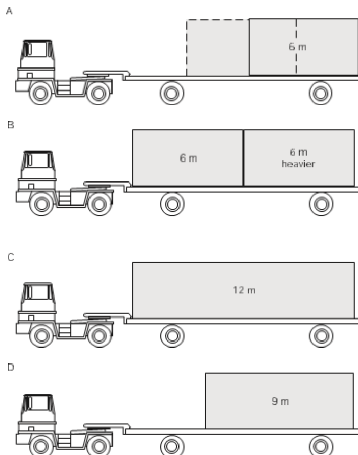
Figure 86 (A, B, C and D). Distribution of load on a trailer
