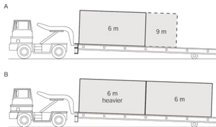
Figure 87 (A and B). Distribution of load on a roll trailer
