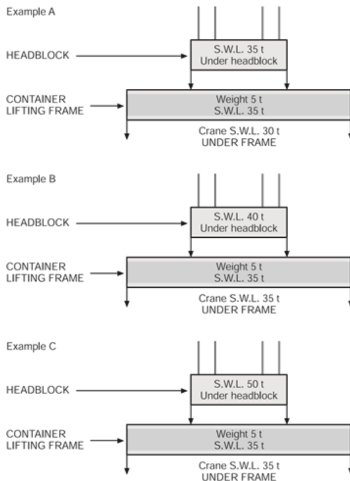
Figure 28. Examples of marking SWL on heavy items of loose gear
