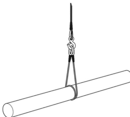
Figure 84. Single sling lift by wrapped choke hitch
