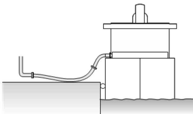
Figure 89. Position of insulating flange in cargo-transfer hose
