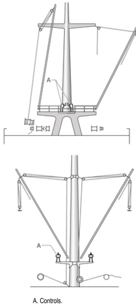
Figure 29. Example of lifting appliance controls – Ships’ derricks
