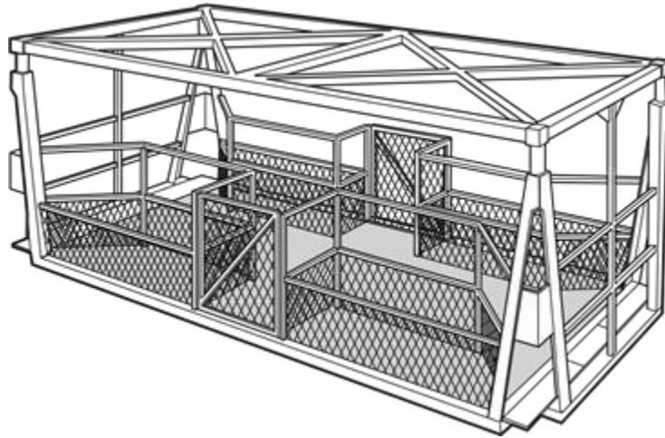
Figure 22. Access or lashing cage
