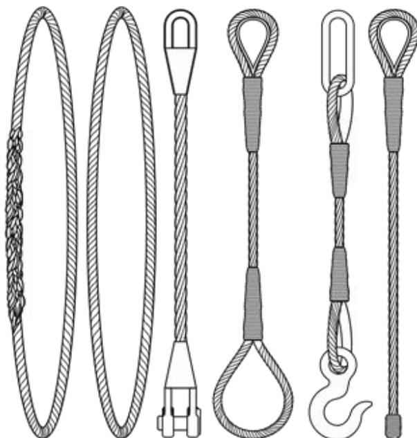
Figure 42. Steel wire slings
