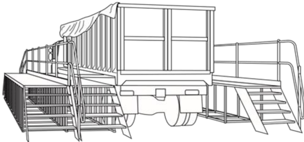
Figure 23. Vehicle sheeting platform
