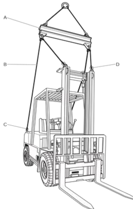
Figure 106. Lifting frame and attachment points for lift truck (all the proper guards have been omitted for clarity)
