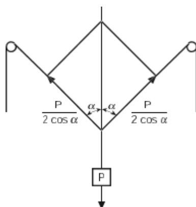
Figure 55. Tension in union purchase cargo falls
