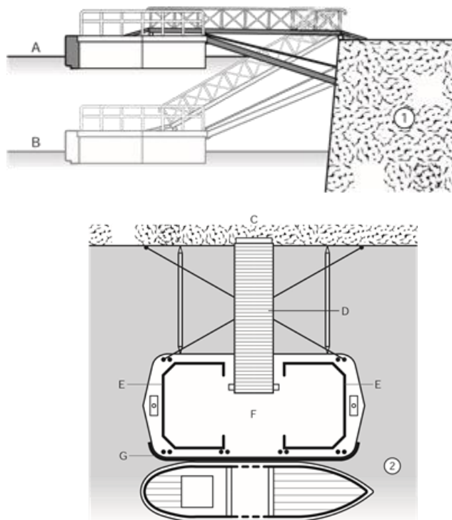
Figure 12. Pontoon landing stage with linkspan or brow
