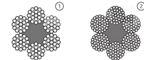
Figure 41. Construction of wire ropes
