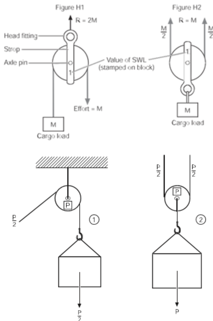
Figure 47. Safe working loads of a single-sheave block
