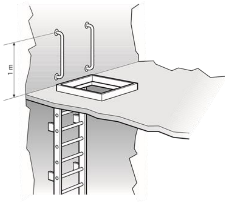
Figure 15. Vertical ladder through opening
