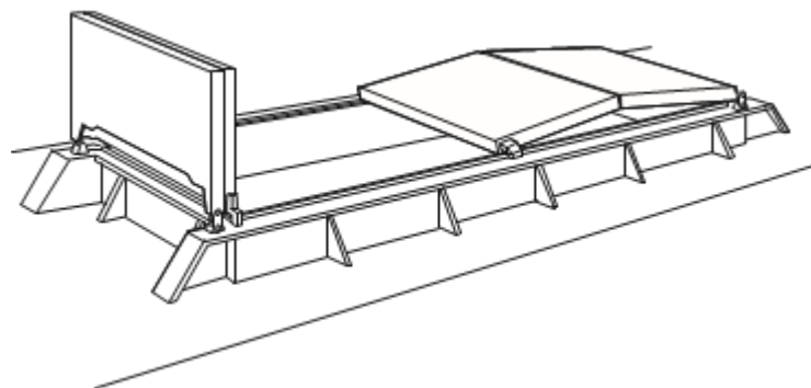
Figure 102. General arrangement for a rolling/sliding hatch cover
