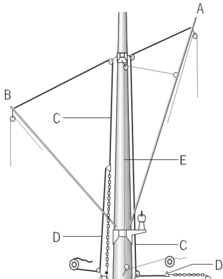
Figure 32. Ships' lifting appliances – A ship's derrick with topping lift and pendant
