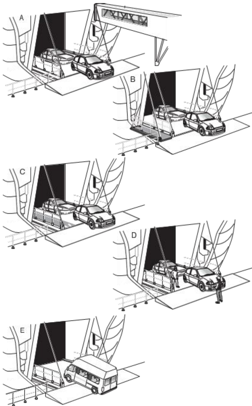
Figure 99. Control of pedestrians on ramps
