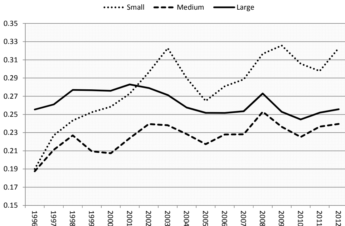
Figure 3: Leverage by firm size
