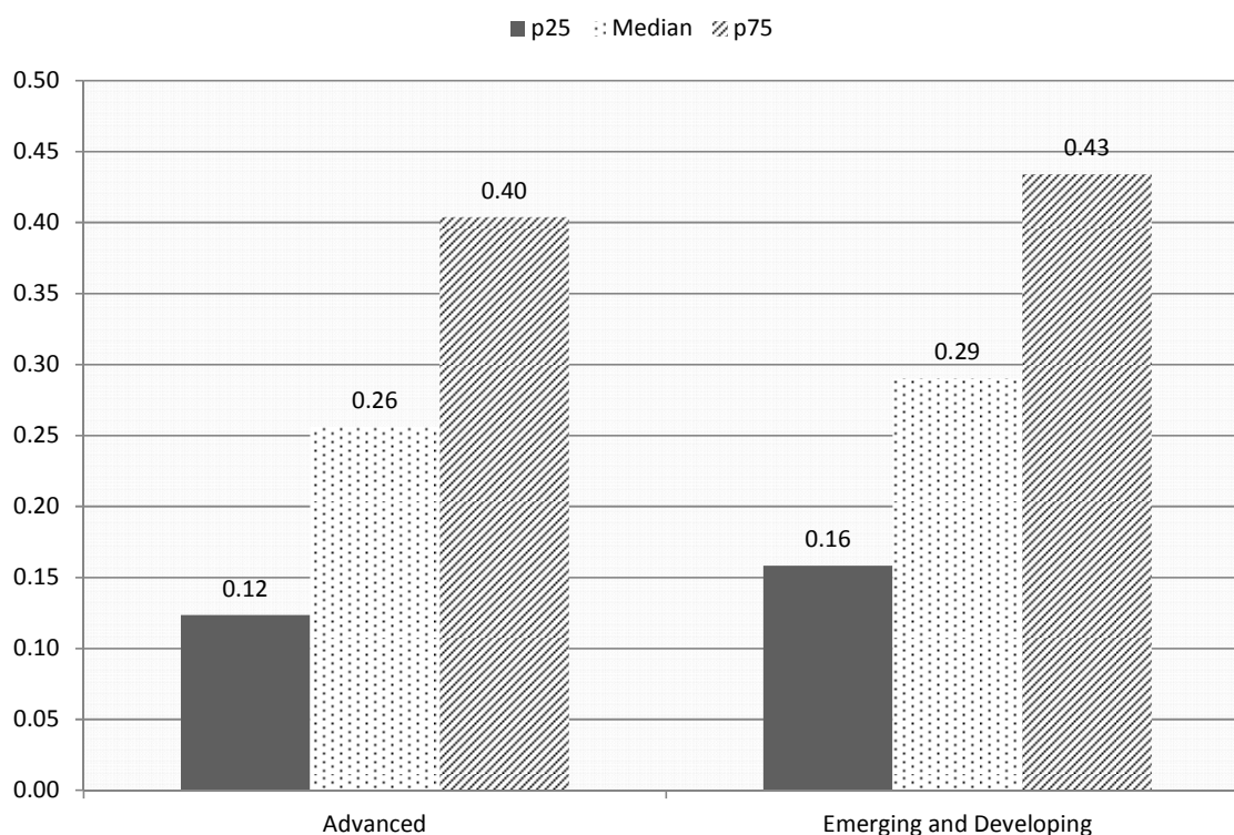
Figure 2: Leverage by income groups
