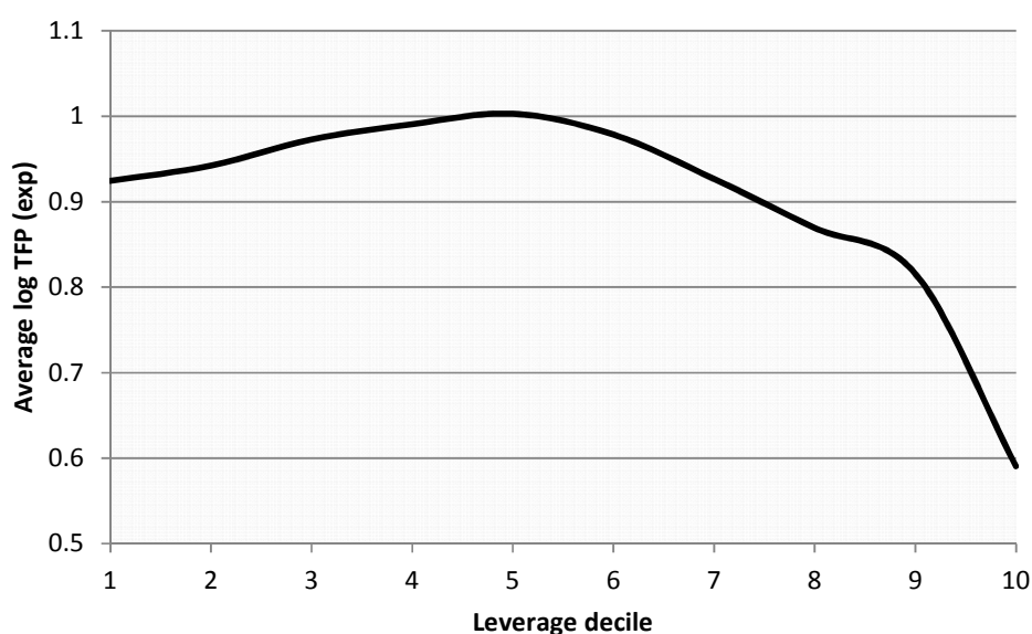
Figure 4: Leverage and TFP
