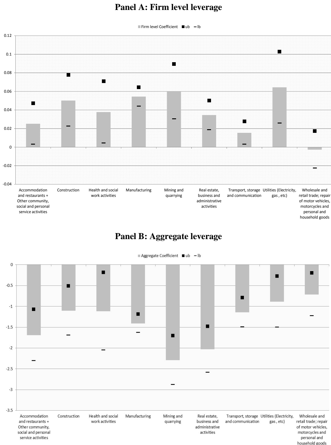
Figure 5: Leverage and TFP by broad sectors
